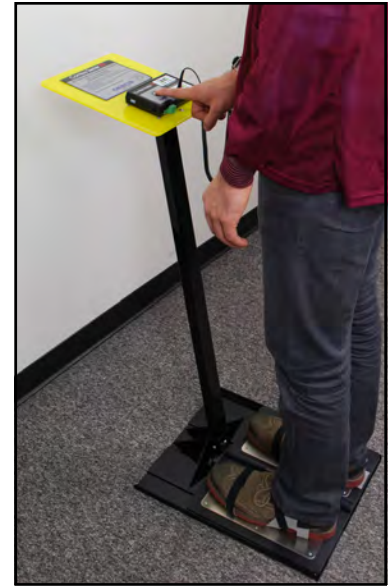
Using the 19279 Combo Tester X3 with Stand
